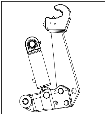
Fig. 6.6: transportstilling
